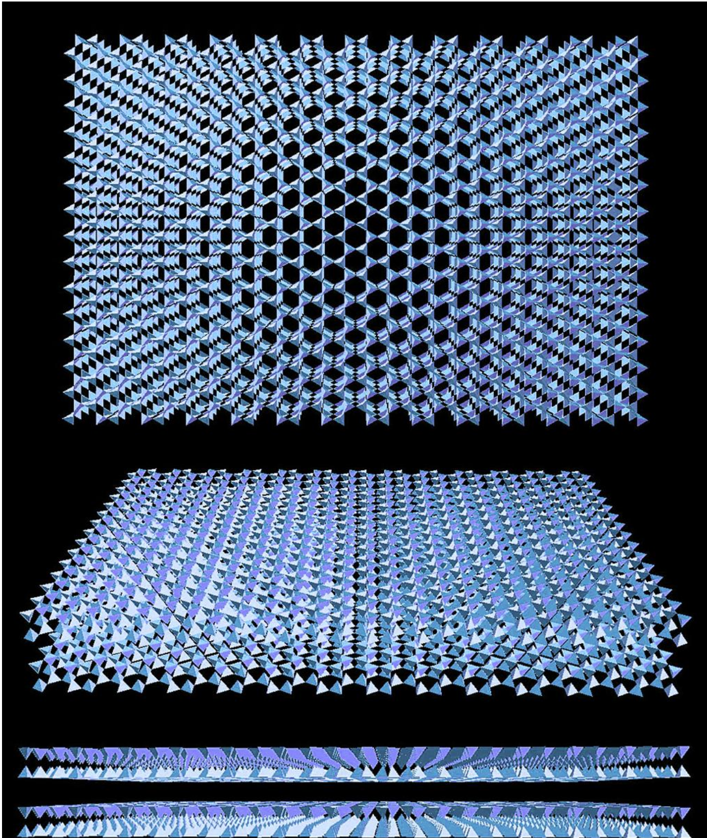
'Sky stone' tetrahedral sheet silicate: poly(siloxonate) [\text{Si}_2\text{O}_5]_n
